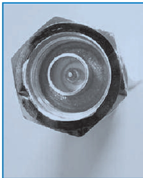
Connector Problems Corroded Connectors Low Quality Connectors Poor Center Pin Contact
