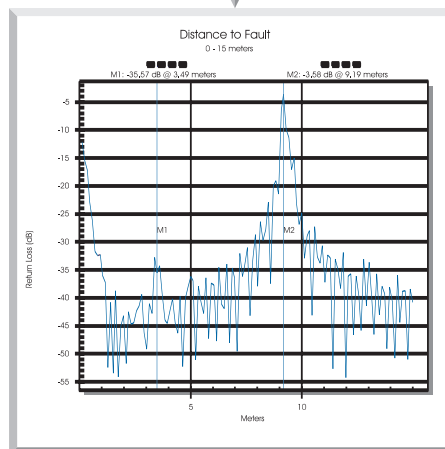
Figure 1. Actual Return Loss vs. Distance
